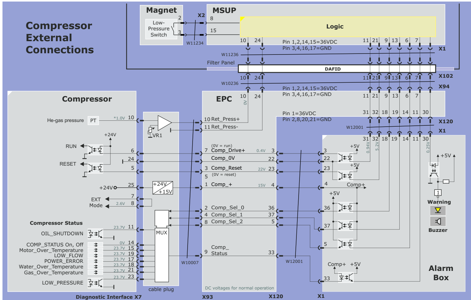
Figure 210 F70 Compressor Control Diagram
