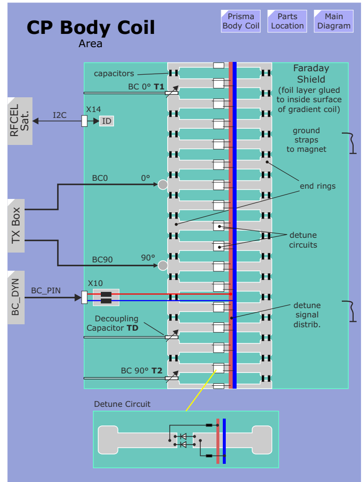
Figure 50 Body Coil Block Diagram
