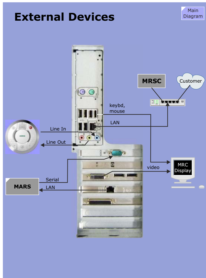
Figure 24 External Devices
