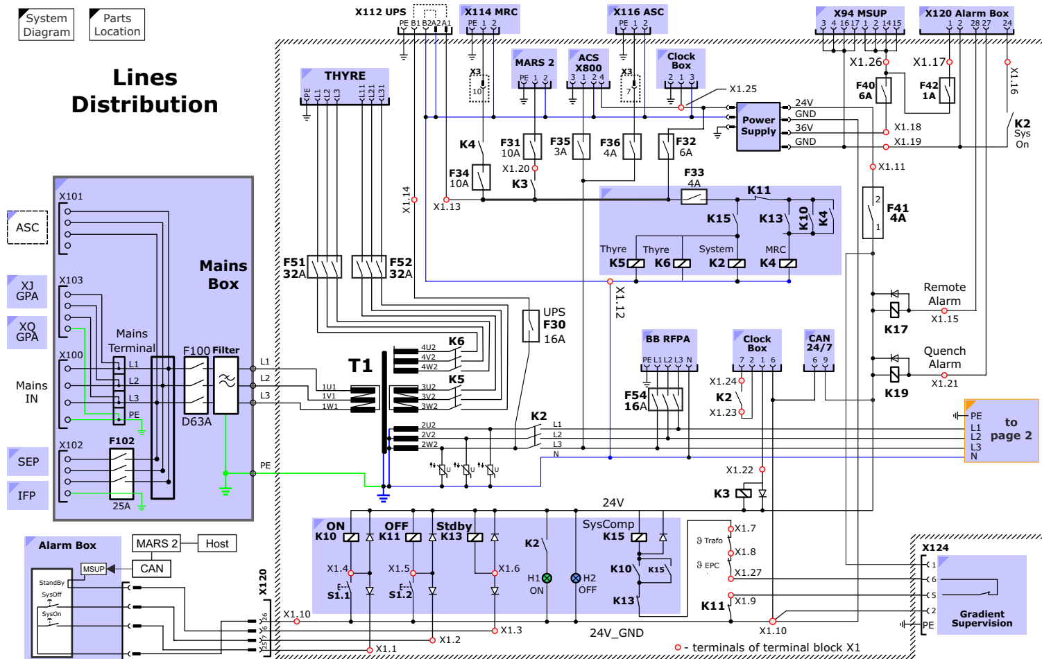
Figure 226 Line Power Distributor Diagram, page 1
