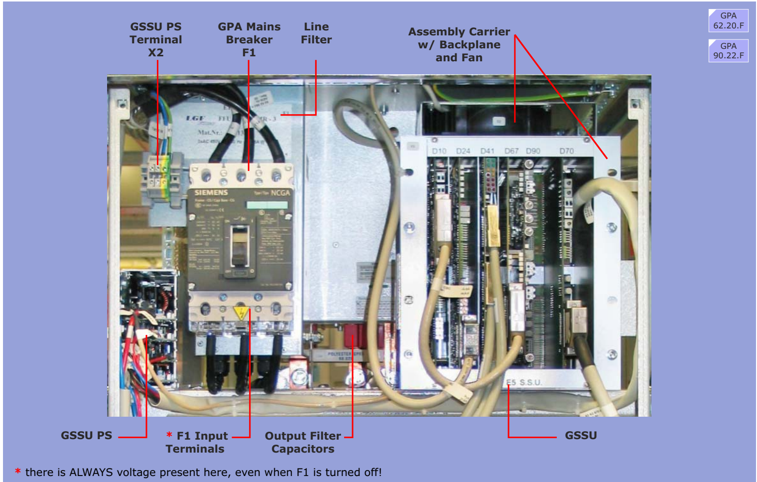
Figure 148 GSSU Layout
