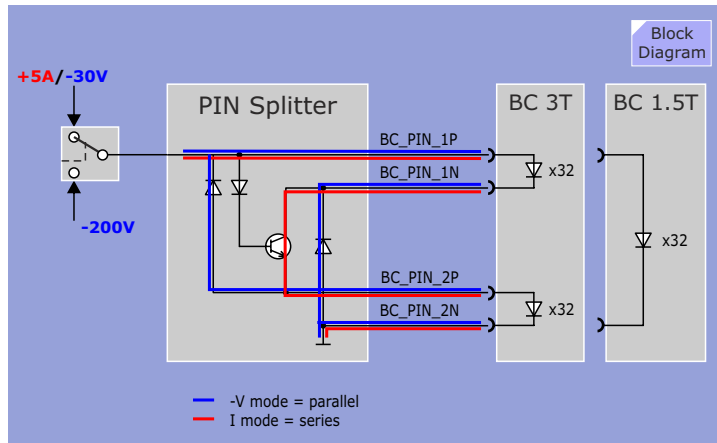
Figure 66 PIN Splitter
