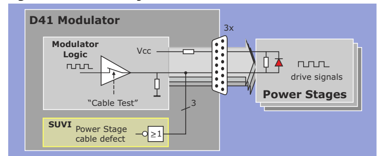
Figure 159 Power Stage Cable Test
