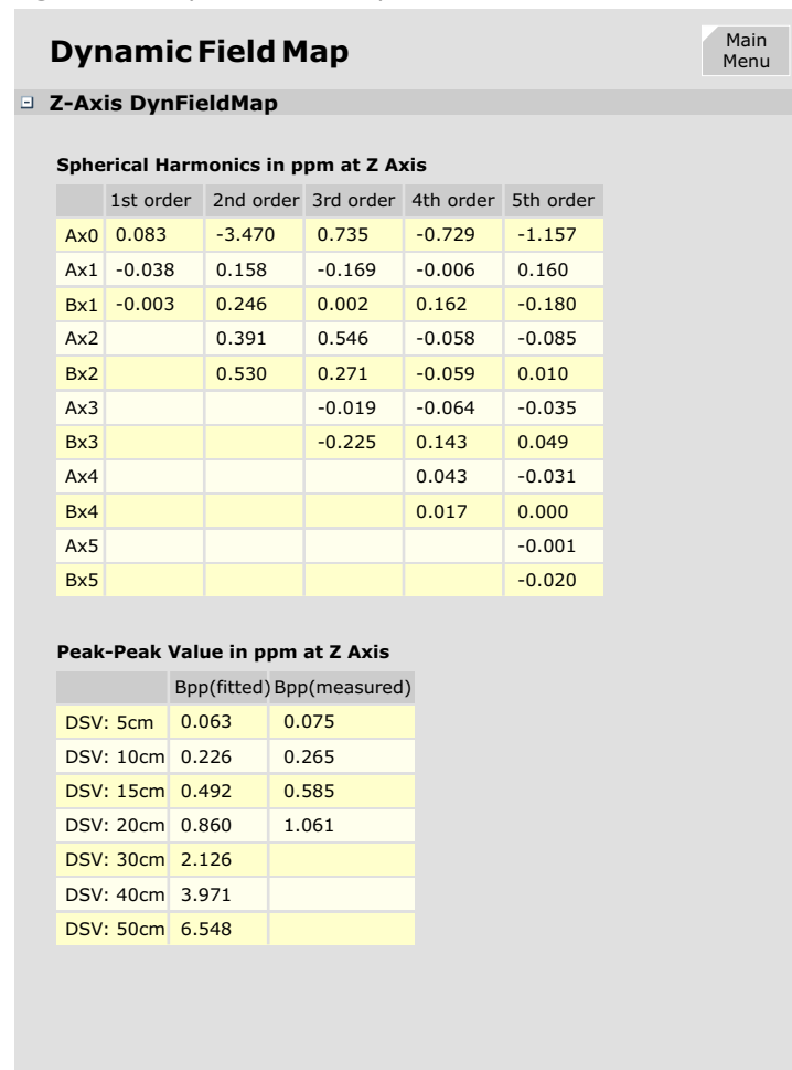
Figure 246 Dynamic Field Map
