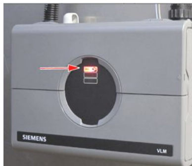
Figure 187 Fire Alarm LED
