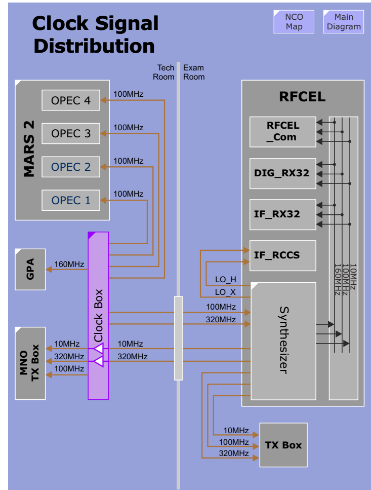
Figure 41 Clock Signal Distribution
