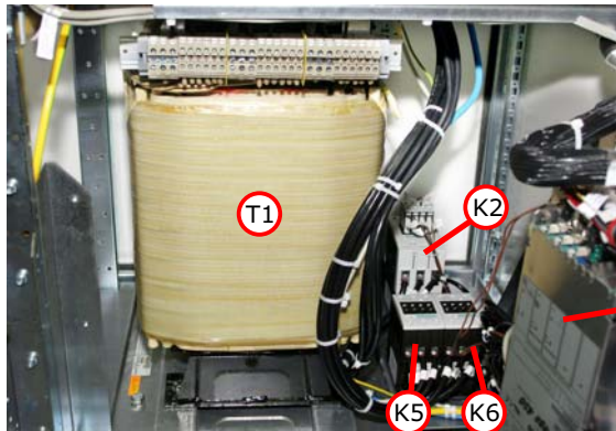
Figure 229 Line Power Distributor Parts Location
