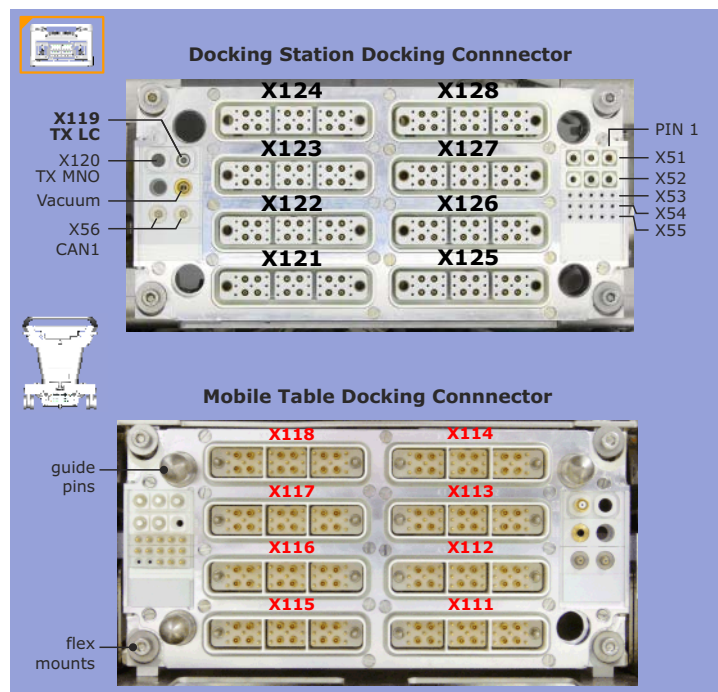
Figure 120 Connector Assemblies
