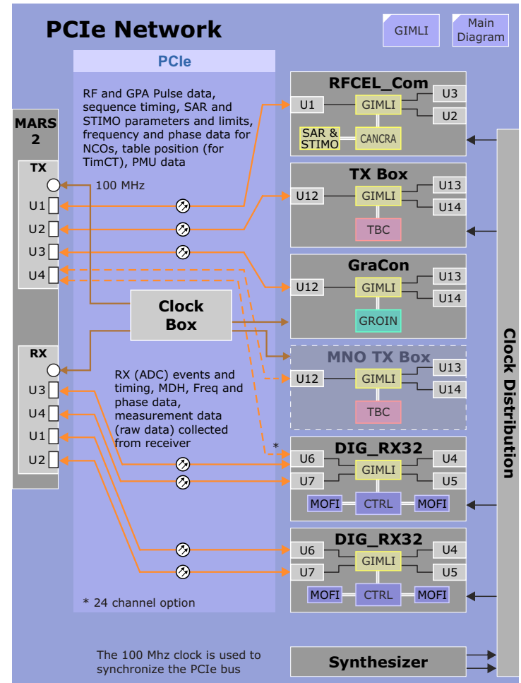
Figure 33 PCIe Network
