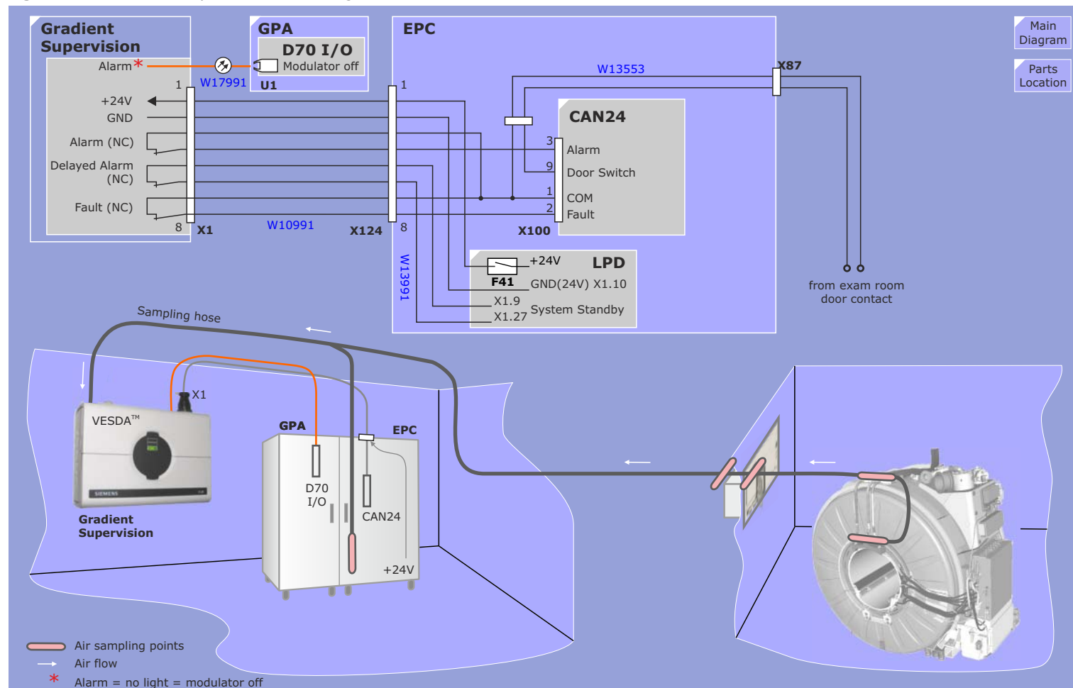
Figure 185 Gradient Supervision Block Diagram
