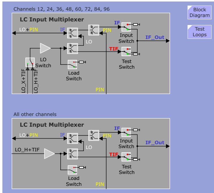
Figure 58 LC Input Multiplexers
