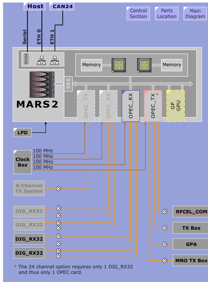
Figure 30 MARS 2 Block Diagram
