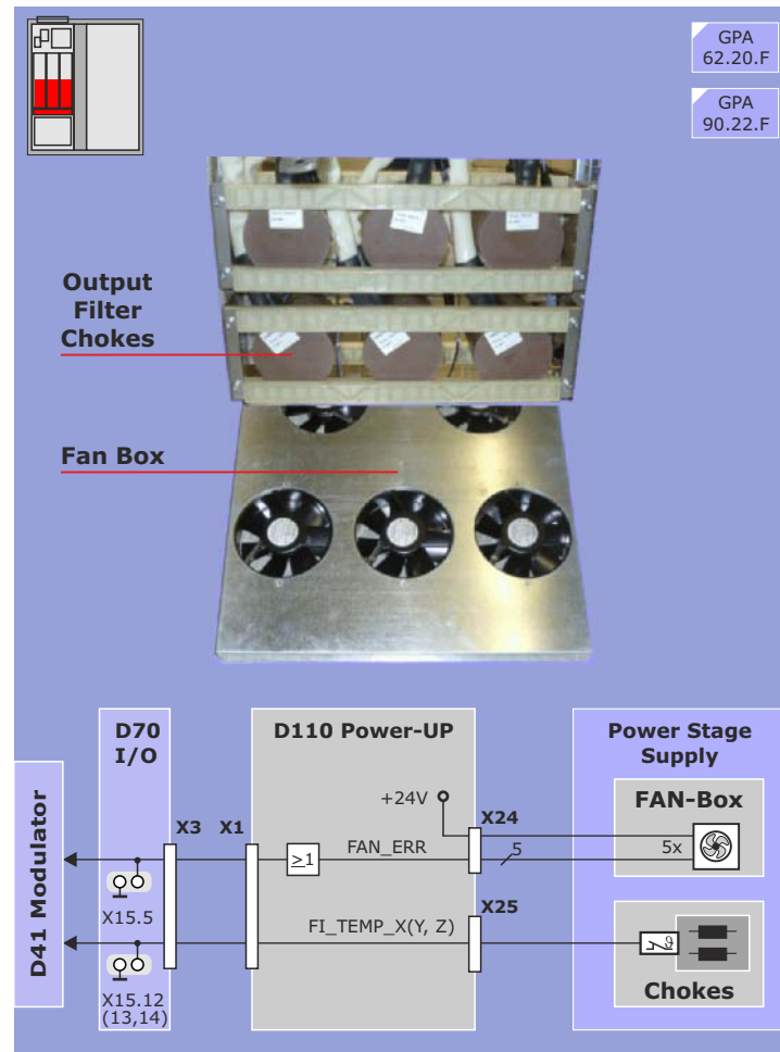
Figure 182 Output Filter-Chokes and Fan Box
