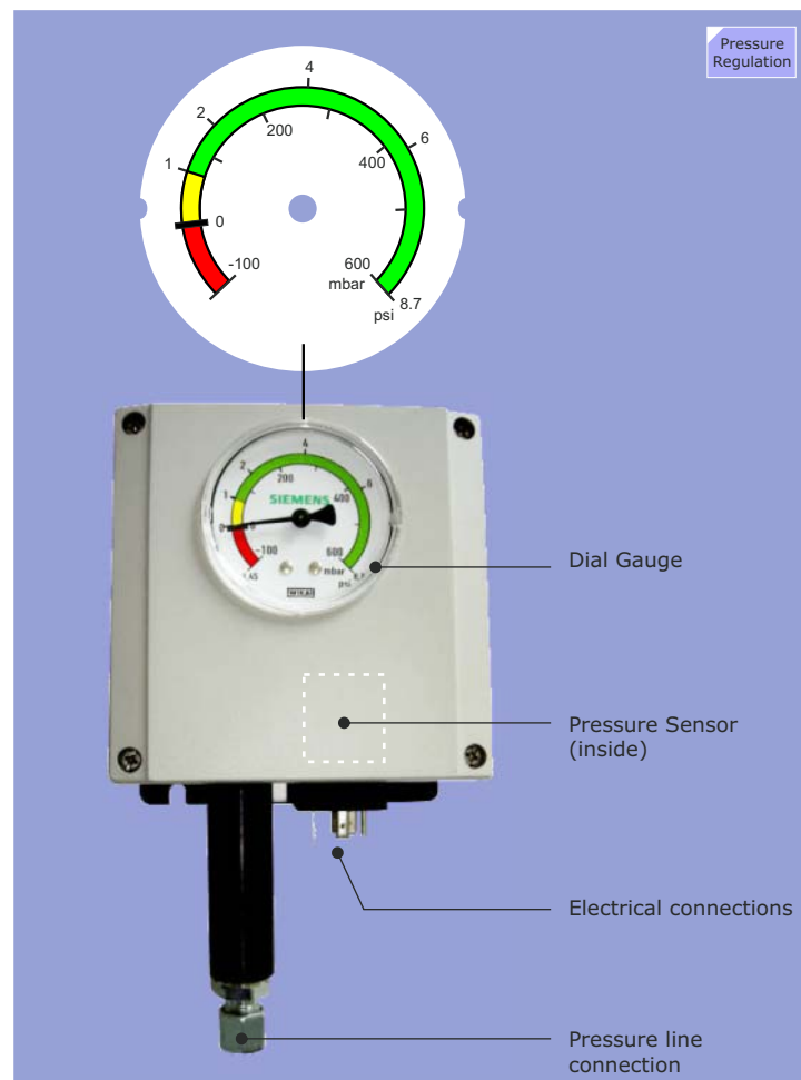
Figure 196 Pressure Display & Control Switch
