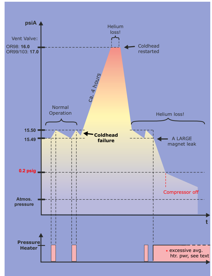
Figure 201 Magnet Pressure Regulation
