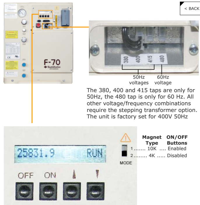
Figure 209 F70 Helium Compressor
