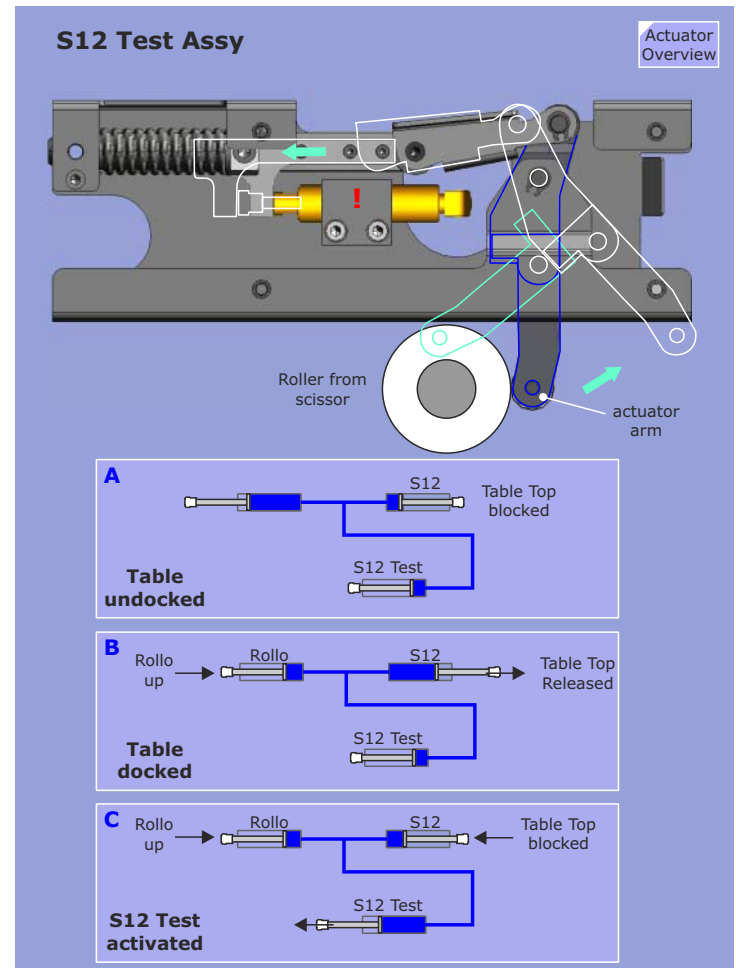
Figure 115 S12 Test Assembly
