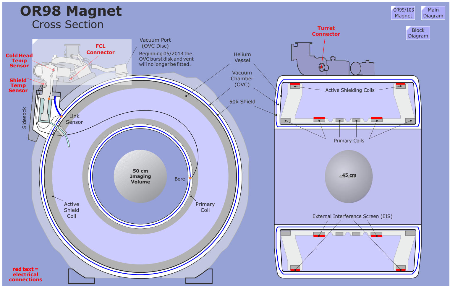
Figure 191 OR98 Magnet - Cross Sectional Diagram
