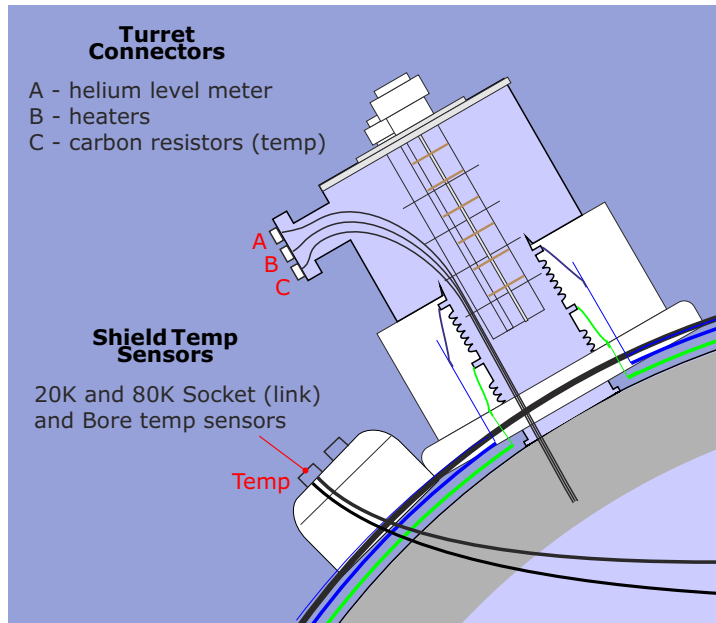
Figure 265 Electrical Connections
