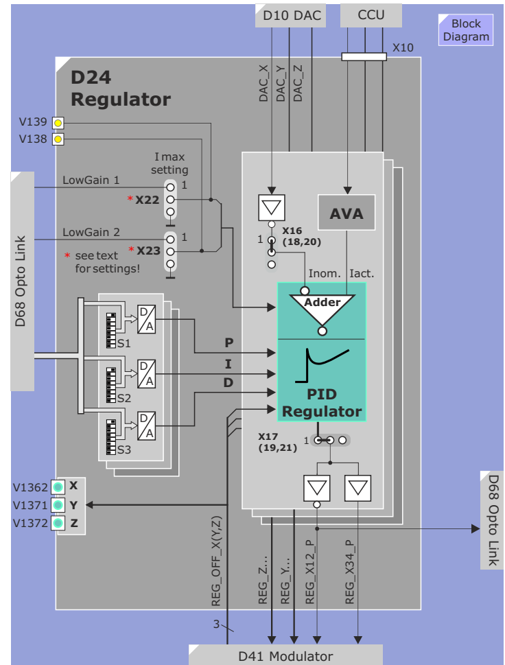
Figure 154 D24 PID Regulator
