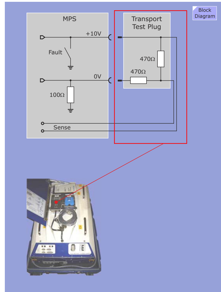
Figure 261 Transport Test Plug
