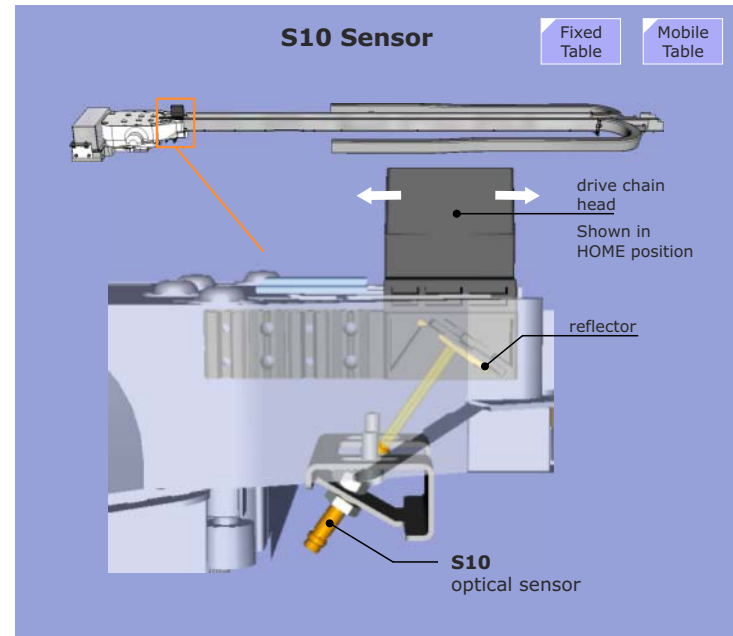
Figure 106 Horizontal HOME Detector S10
