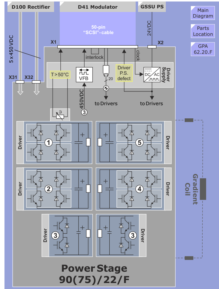
Figure 174 90/22/F Power Stage Block Diagram
