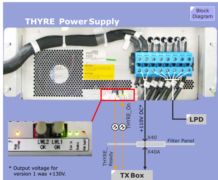
Figure 49 THYRE Power Supply
