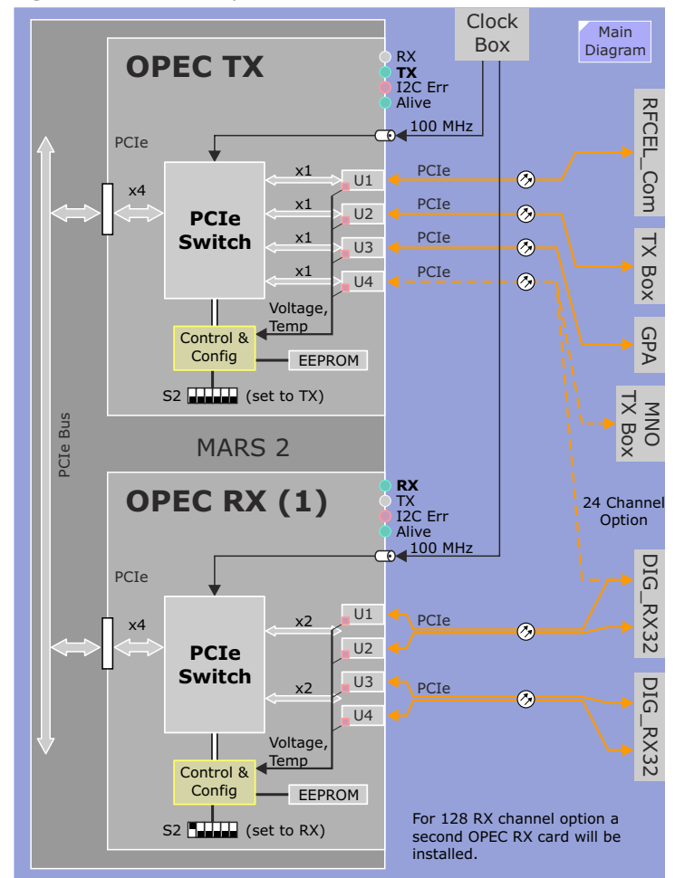
Figure 31 OPEC - Optical PCIe Card
