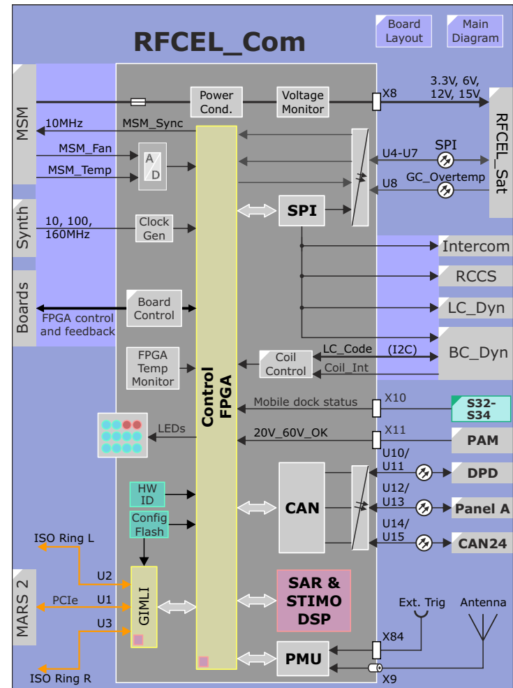
Figure 71 RFCEL_Com Block Diagram
