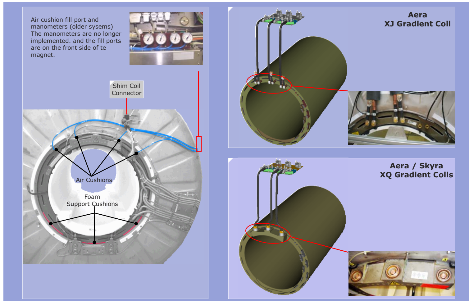
Figure 183 Gradient Coil and Suspension)
