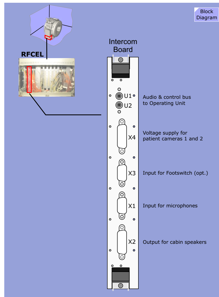
Figure 138 Intercom Board Front View
