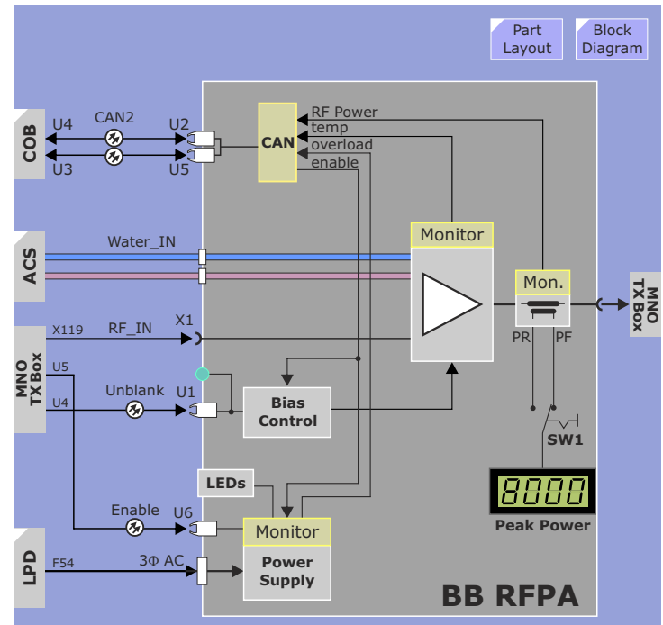
Figure 89 BB RFPA
