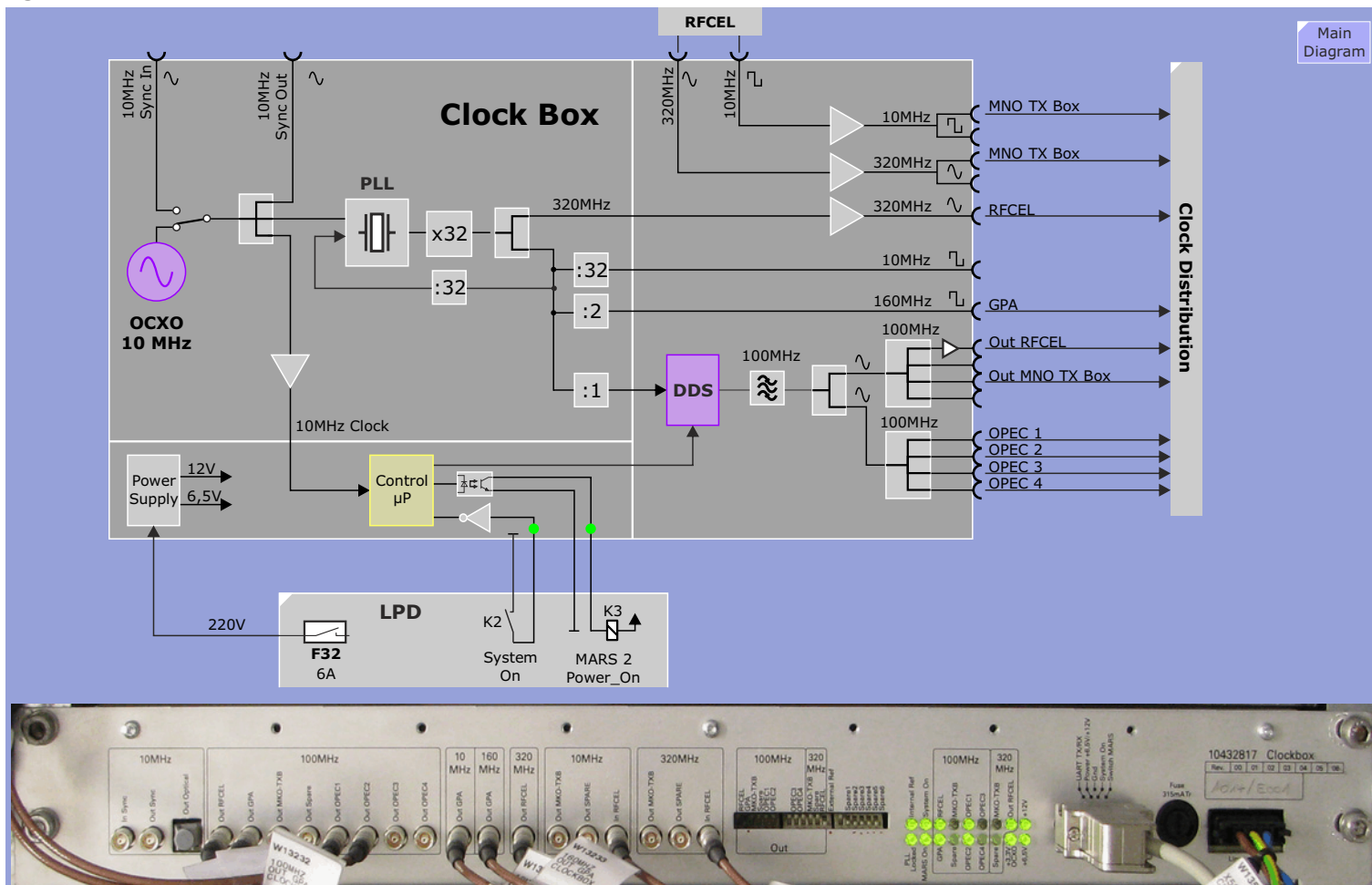
Figure 42 Clock Box
