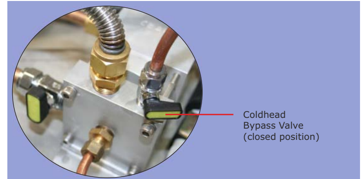
Figure 212 Cold Head bypass valve CLOSED
