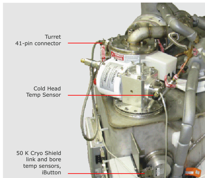
Figure 195 Electrical Connectors
