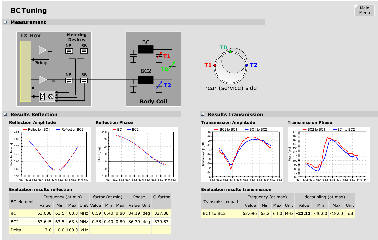
Figure 235 Body Coil Resonant Frequency and De-coupling Adjustments
