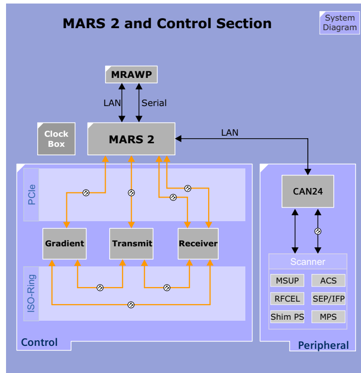
Figure 27 MARS and Control Overview Diagram
