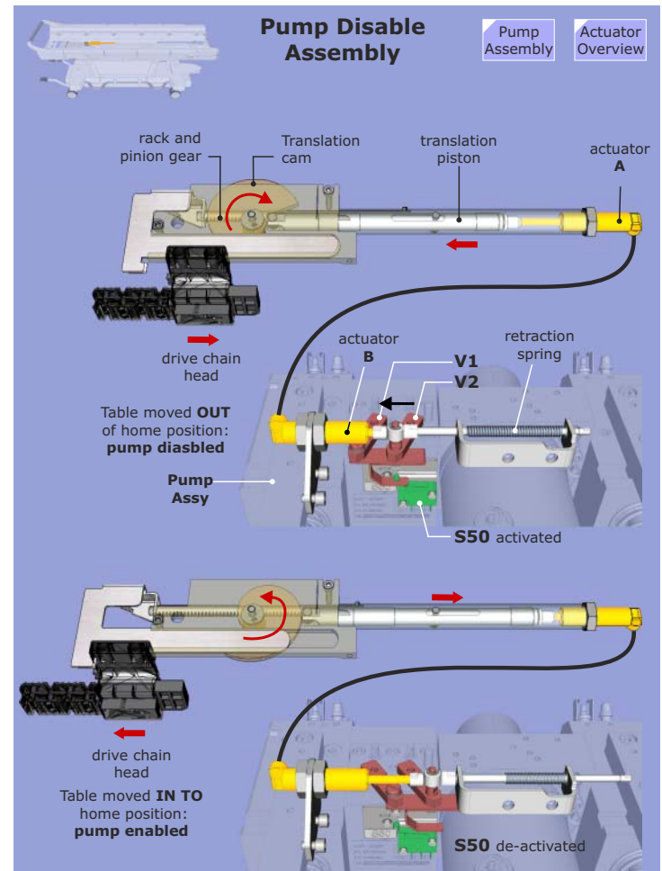
Figure 113 Pump Disable
