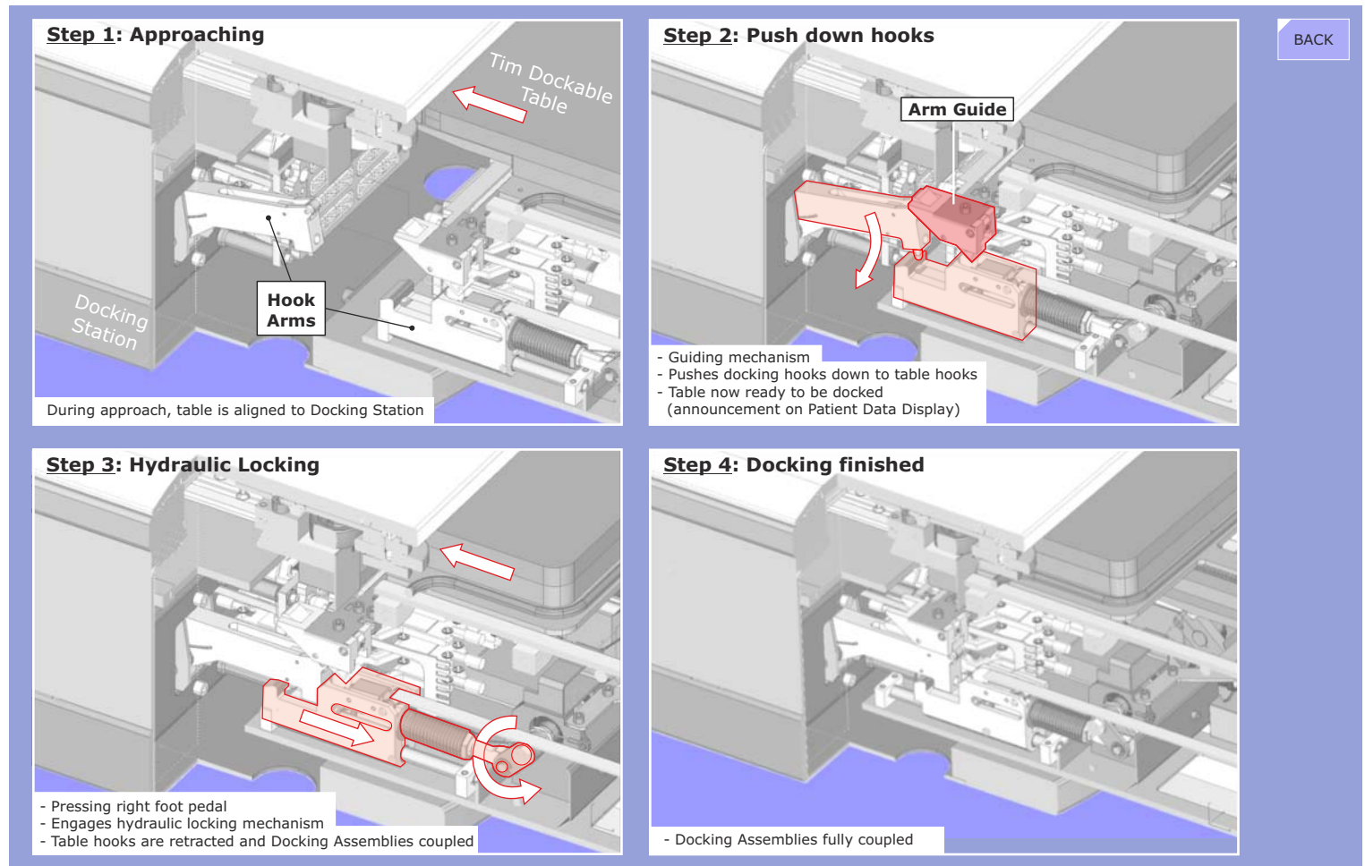
Figure 118 Docking Process
